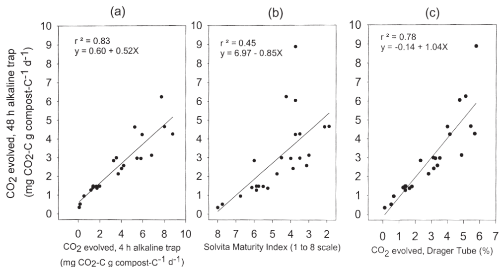
FIGURE 3. Relationships between \text{CO}_2 evolved using 4 h methods vs. \text{CO}_2 evolved using 48 h alkaline trap method. Four hour methods: alkaline trap (a), Solvita (b), Dräger, percent \text{CO}_2 as read from tube (c). Combined data from winter and spring trials. Each data point represents one windrow-date mean ( n = 4 ) for independent composite samples collected within a single windrow.
